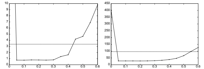
Figure 2. The average error rate (left) and number of support vectors (right) as a function of the diffusion coefficient \beta on the Mushroom data set. The horizontal line is the baseline performance using the Hamming kernel.
