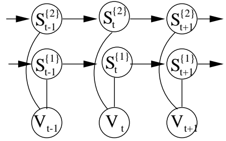
Figure 2: Product of HMM’s
