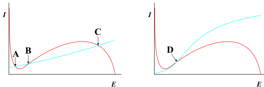
Figure 1: Two possible sets of nullclines. In both figures, the red curve is the excitatory nullcline and the blue curve is the inhibitory one.
