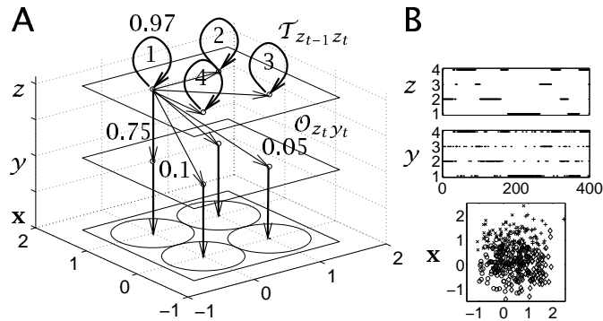
Figure 1: Generative model. A) Three-layer model z \in \{1-4\} \Rightarrow y \in \{1-4\} \Rightarrow \mathbf{x} \in \mathbb{R}^2 with dynamics ( \mathcal{T} ) in the z layer ( P[z_t = z_{t-1}] = 0.97 ), a probabilistic mapping ( \mathcal{O} ) from z \rightarrow y ( P[y_t = z_t | z_t] = 0.75 ), and a Gaussian model p[\mathbf{x} | y] with means at the corners of the unit square and standard deviation 0.5 in each direction. The model is rotationally invariant; only some of the links are shown for convenience. B) Sample sequence showing the slow dynamics in z ; the stochastic mapping into y and the substantial overlap in \mathbf{x} (different symbols show samples from the different Gaussians shown in A).
