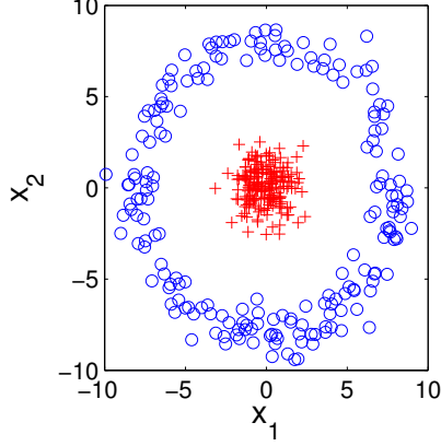
Figure 1: Ring dataset
