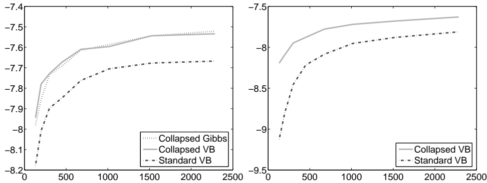
Figure 2: Left: test set per word log probabilities. Right: per word variational bounds. Both as functions of the number of documents for KOS.
